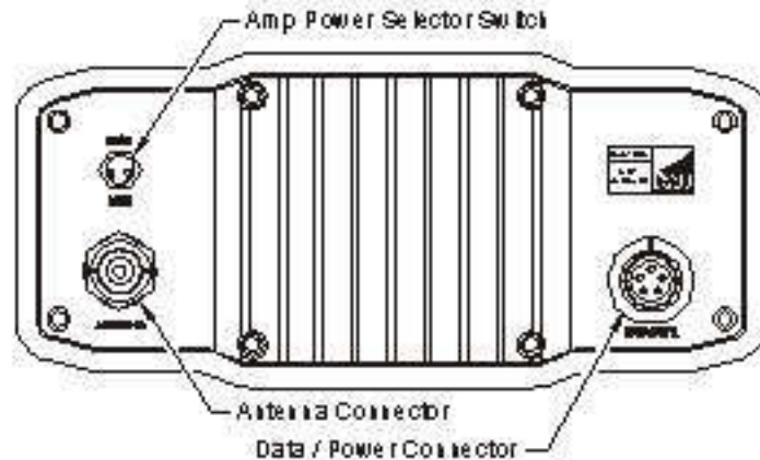
Figure 2 - PDL High Power Base Rear Panel
